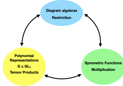
Figure 8: A diagram representing how the mathematical ideas mentioned in this paper are related.
