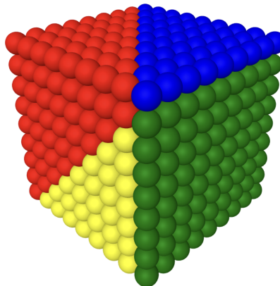
Figure 5: A combinatorial view of the decomposition of V^{\otimes 3} into GL_9 representations.
