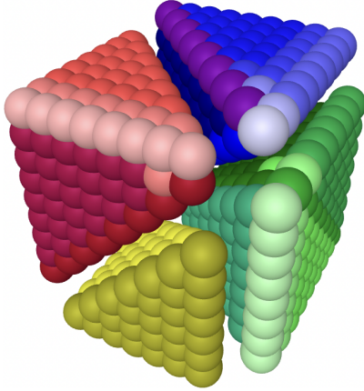
Figure 6: A combinatorial view of the decomposition of V^{\otimes 3} into GL_9 representations by primary colors and then the restriction of those into S_9 representations by the different shades of those regions.
