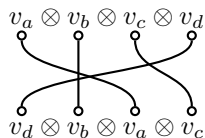
Figure 4: Visualization of the right action of (1, 3, 4) in S_4 on a tensor in V^{\otimes 4} .
